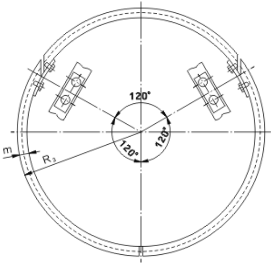
■ U型套管用中間圈 Center Gland for Collar
